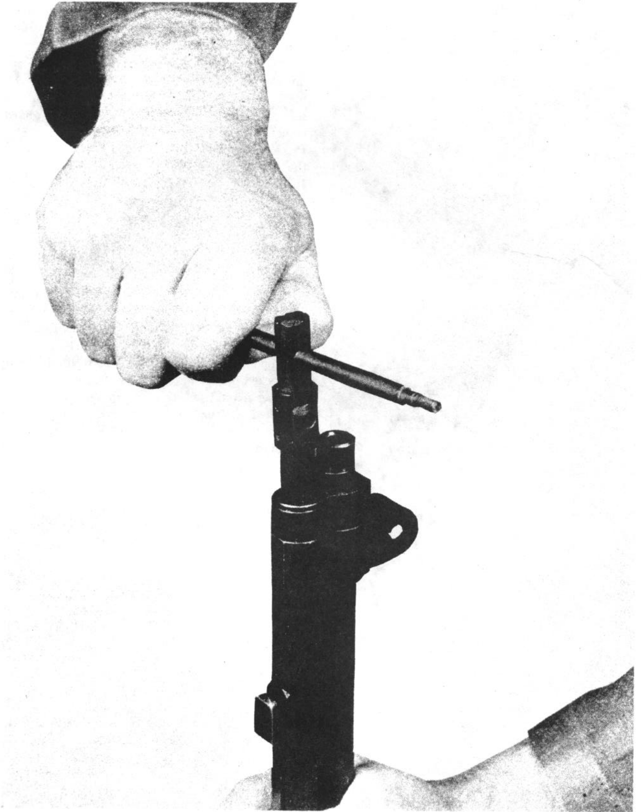
Figure 8. Removing the gas cylinder lock screw.
