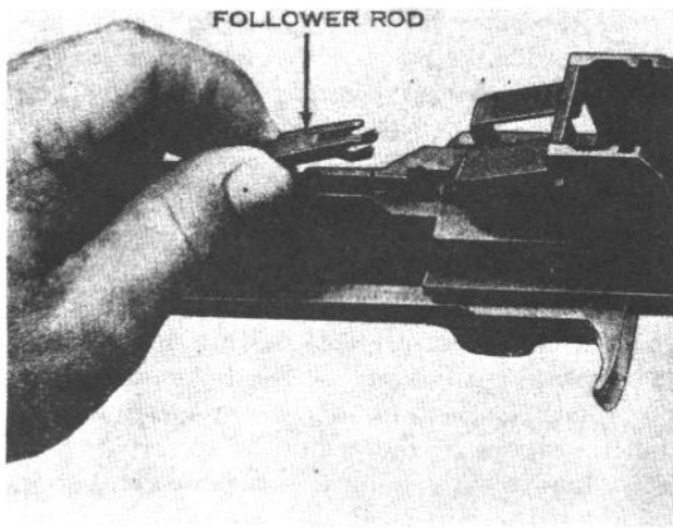
Figure 4. Removing the follower rod and operating rod spring.
