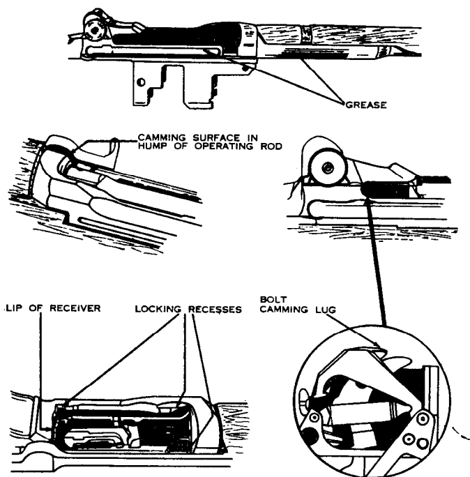
Figure 33. Points to apply rifle grease.
