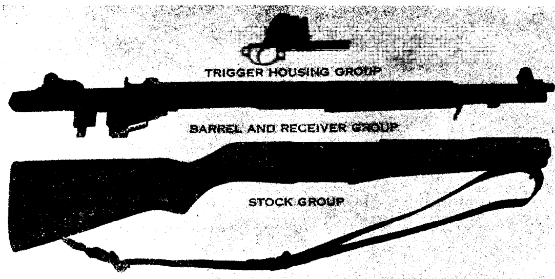
Figure 2. The three main groups.
