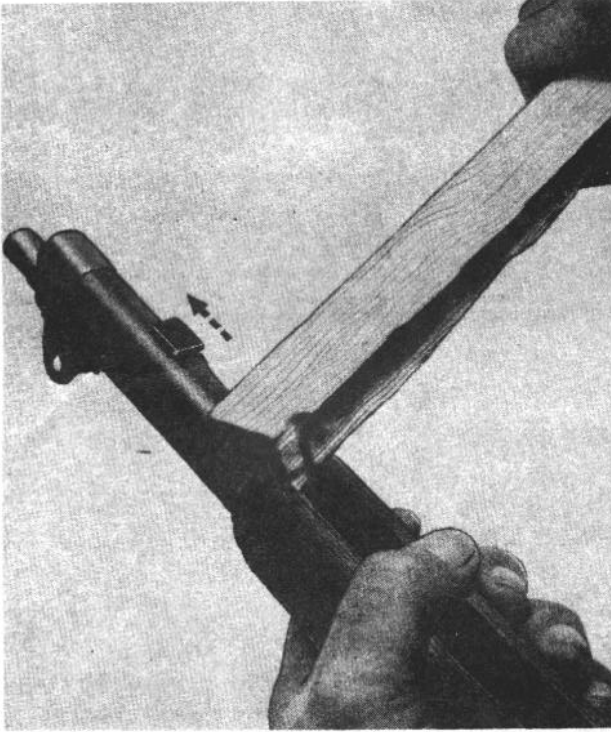
Figure 9. Removing the gas cylinder.
