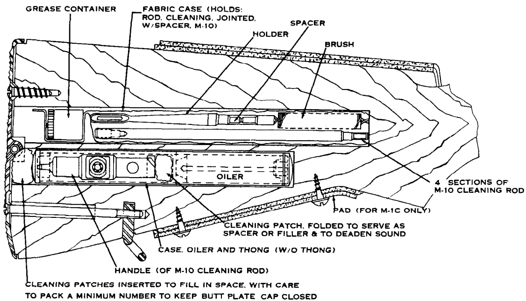
Figure 35. Stowage of accessories in butt stock of M1 and M1C rifles.
