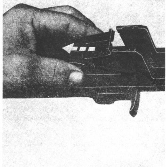
Figure 6. Removing the bullet guide, follower arm, and operating rod catch assembly.
