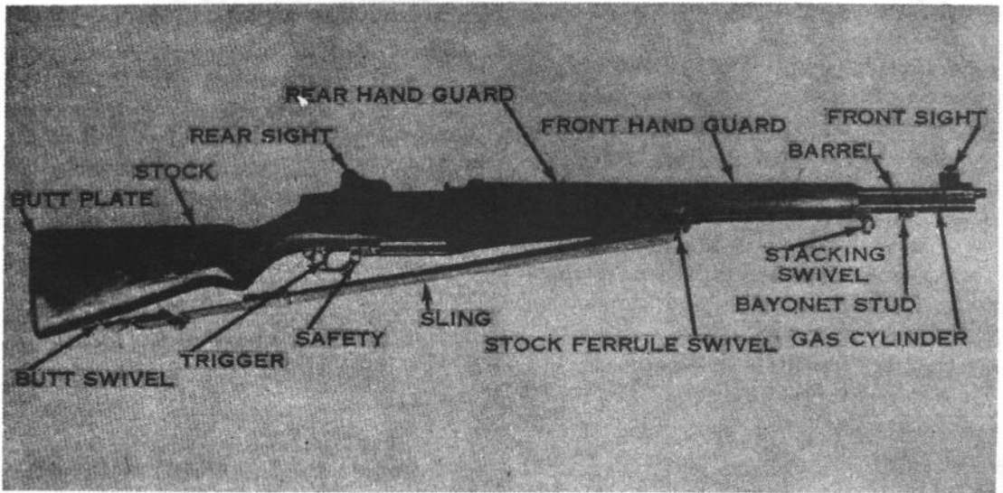
Figure 1. U.S. rifle, caliber .30, M1.
