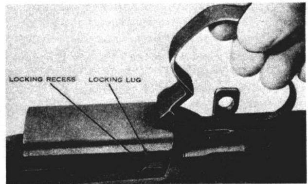
Figure 18. Replacing the trigger housing group.
