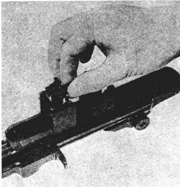
Figure 12. Replacing the follower assembly.
