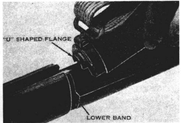
Figure 17. Replacing the stock on the barrel and receiver group.
