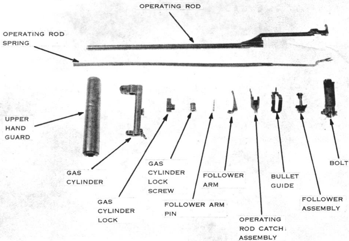
Figure 10. Parts of the barrel and receiver group in the order of disassembly.
