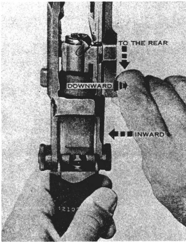
Figure 11. Replacing the operating rod.
