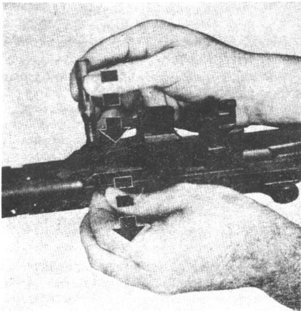
Figure 5. Removing the follower arm pin.
