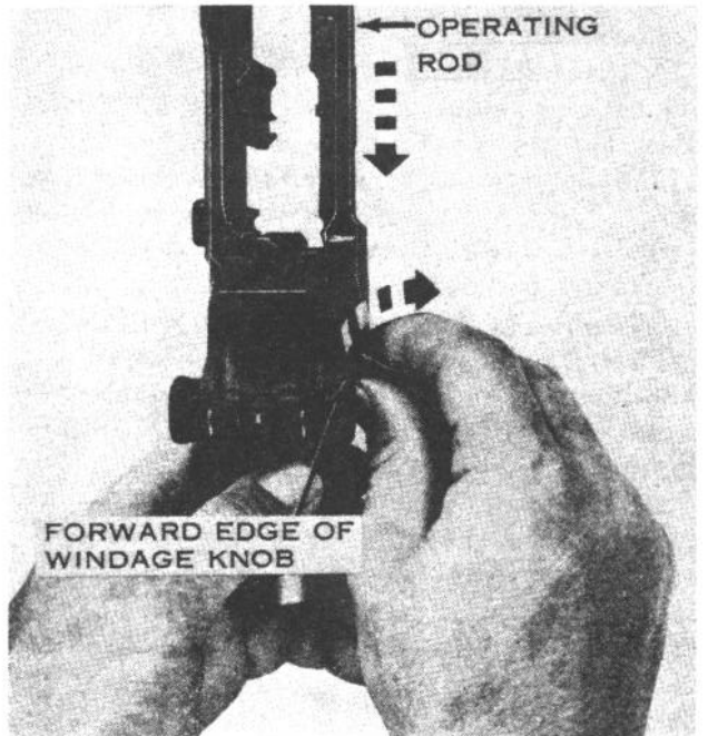
Figure 7. Removing the operating rod.
